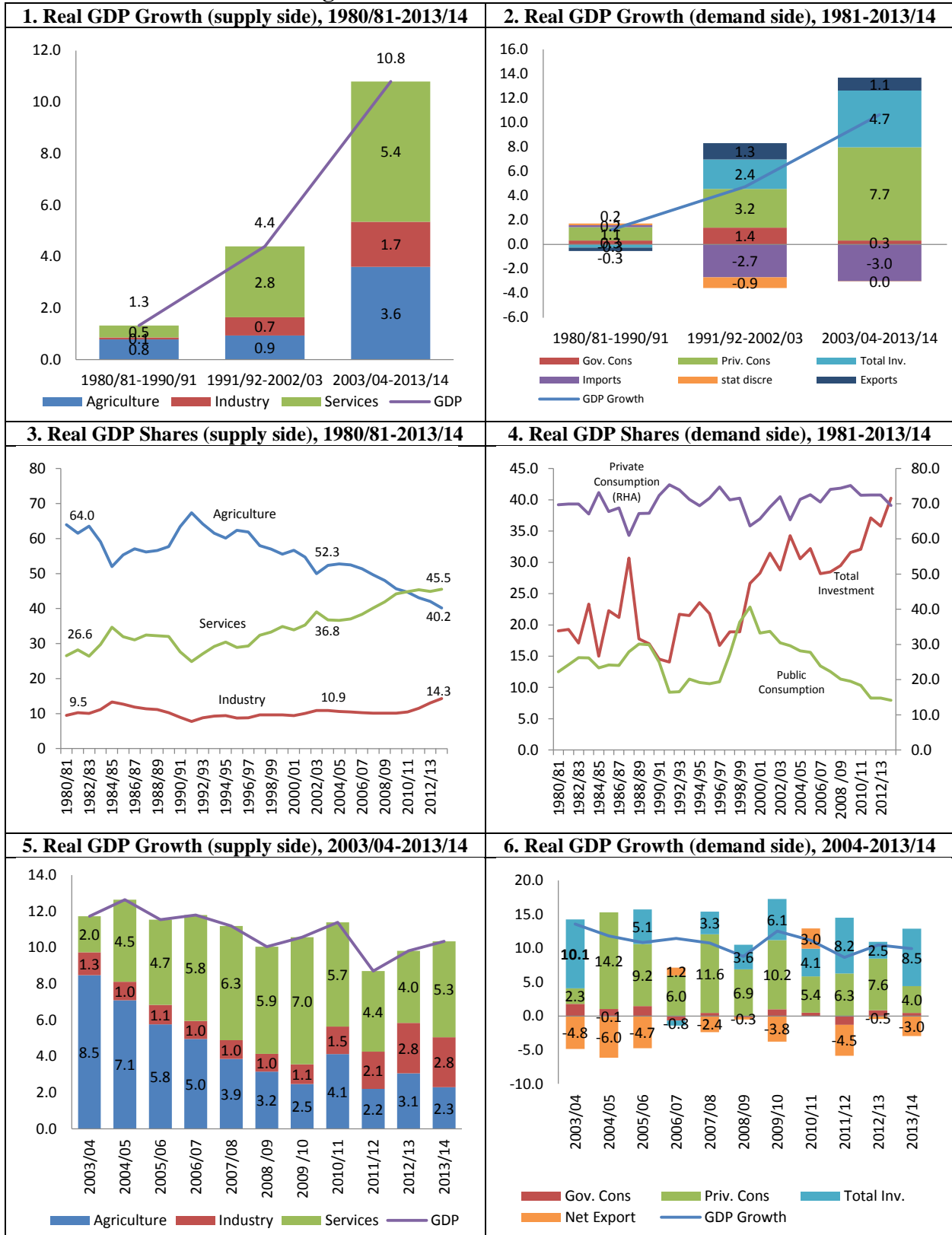
Figure 1.3 Growth Characteristics
