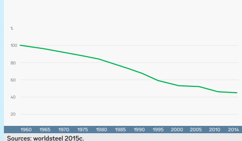
Figure B1.1.2 Indexed Global Energy Consumption/ Tonne of Crude Steel Production
