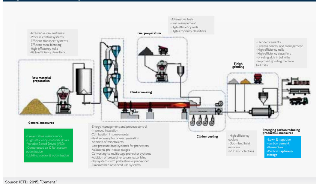
Figure 1.10 Cement-making Process and Associated Low-carbon Interventions
