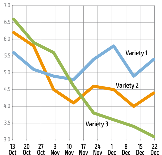
Figure 2.5 Grain yields of elite wheat cultivars by planting date, Bihar and Madhya Pradesh, India (t/ha)
