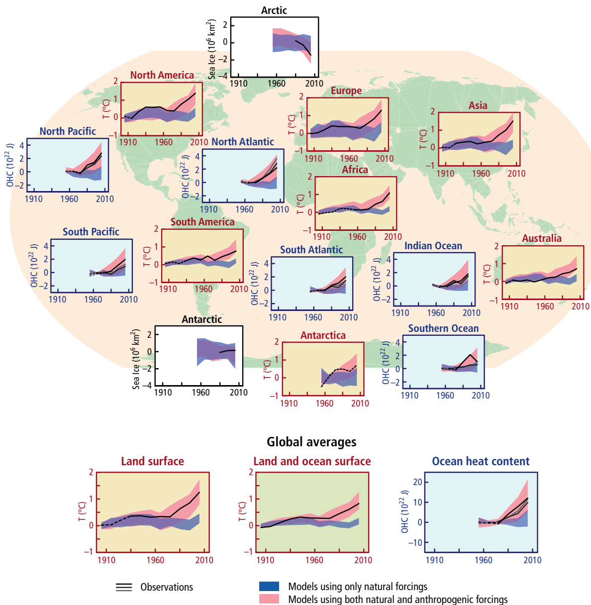
Figure 1.10 | Comparison of observed and simulated change in continental surface temperatures on land (yellow panels), Arctic and Antarctic September sea ice extent (white panels), and upper ocean heat content in the major ocean basins (blue panels). Global average changes are also given. Anomalies are given relative to 1880–1919 for surface temperatures, to 1960–1980 for ocean heat content, and to 1979–1999 for sea ice. All time series are decadal averages, plotted at the centre of the decade. For temperature panels, observations are dashed lines if the spatial coverage of areas being examined is below 50%. For ocean heat content and sea ice panels, the solid lines are where the coverage of data is good and higher in quality, and the dashed lines are where the data coverage is only adequate, and, thus, uncertainty is larger (note that different lines indicate different data sets; for details, see WGI Figure SPM.6). Model results shown are Coupled Model Intercomparison Project Phase 5 (CMIP5) multi-model ensemble ranges, with shaded bands indicating the 5 to 95% confidence intervals. {WGI Figure SPM 6; for detail, see WGI Figure TS.12}
