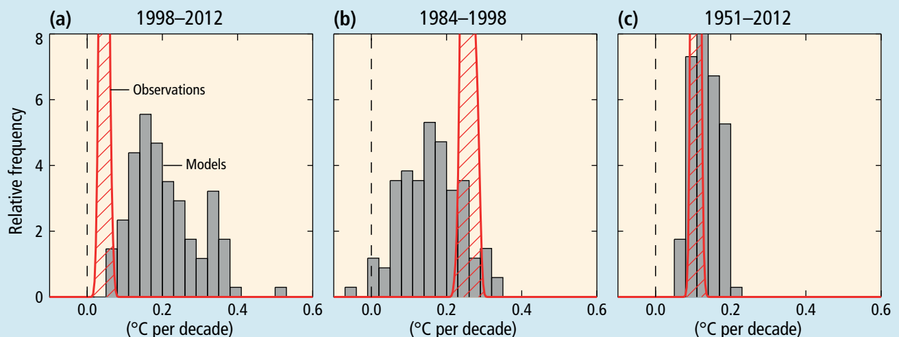
Box 1.1, Figure 1 | Trends in the global mean surface temperature over the periods from 1998 to 2012 (a), 1984 to 1998 (b), and 1951 to 2012 (c), from observations (red) and the 114 available simulations with current-generation climate models (grey bars). The height of each grey bar indicates how often a trend of a certain magnitude (in °C per decade) occurs among the 114 simulations. The width of the red-hatched area indicates the statistical uncertainty that arises from constructing a global average from individual station data. This observational uncertainty differs from the one quoted in the text of Section 1.1.1; there, an estimate of natural internal variability is also included. Here, by contrast, the magnitude of natural internal variability is characterised by the spread of the model ensemble. {based on WGI Box 9.2, Figure 1}
