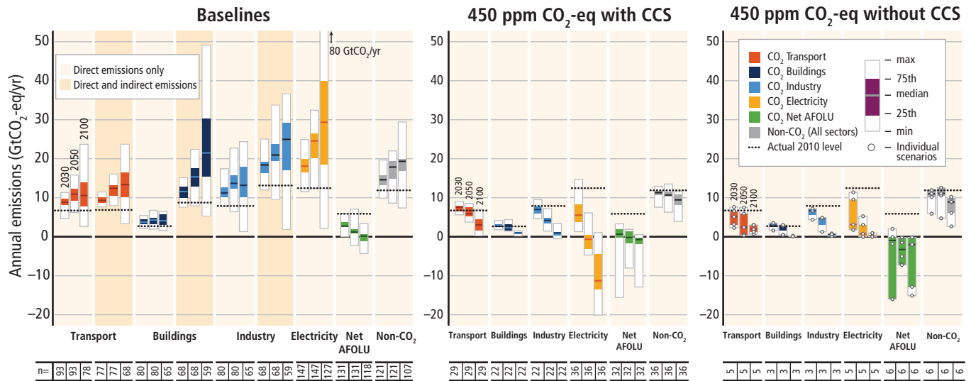
Figure 4.1 | Carbon dioxide (CO 2 ) emissions by sector and total non-CO 2 greenhouse gas (GHG) emissions (Kyoto gases) across sectors in baseline (left panel) and mitigation scenarios that reach about 450 (430 to 480) ppm CO 2 -eq ( likely to limit warming to 2°C above pre-industrial levels) with carbon dioxide capture and storage (CCS, middle panel) and without CCS (right panel). Light yellow background denotes direct CO 2 and non-CO 2 GHG emissions for both the baseline and mitigation scenarios. In addition, for the baseline scenarios, the sum of direct and indirect emissions from the energy end-use sectors (transport, buildings and industry) is also shown (dark yellow background). Mitigation scenarios show direct emissions only. However, mitigation in the end-use sectors leads also to indirect emissions reductions in the upstream energy supply sector. Direct emissions of the end-use sectors thus do not include the emission reduction potential at the supply-side due to, for example, reduced electricity demand. Note that for calculating the indirect emissions only electricity emissions are allocated from energy supply to end-use sectors. The numbers at the bottom of the graphs refer to the number of scenarios included in the range, which differs across sectors and time due to different sectoral resolution and time horizon of models. Note that many models cannot reach concentrations of about 450 ppm CO 2 -eq by 2100 in the absence of CCS, resulting in a low number of scenarios for the right panel. Negative emissions in the electricity sector are due to the application of bioenergy with carbon dioxide capture and storage (BECCS). ‘Net’ agriculture, forestry and other land use (AFOLU) emissions consider afforestation, reforestation as well as deforestation activities. {WGIII Figure SPM.7, Figure TS.15}
