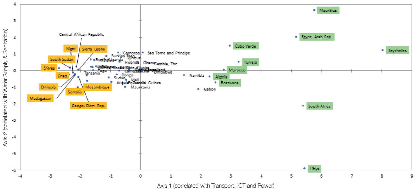
Figure 6. Principal Component Analysis Scatterplot
